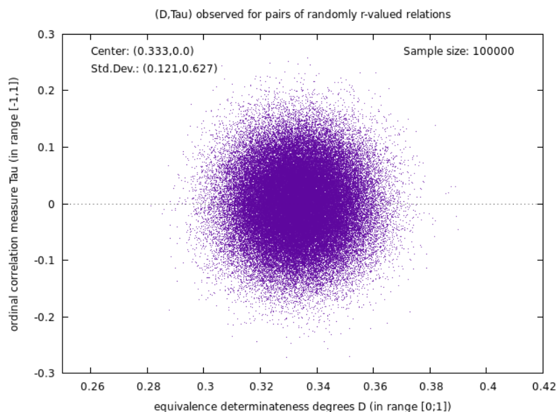
Figure 1: Scatter plot of (d, \tau) for pairs of randomly r -valued relations of order 20
