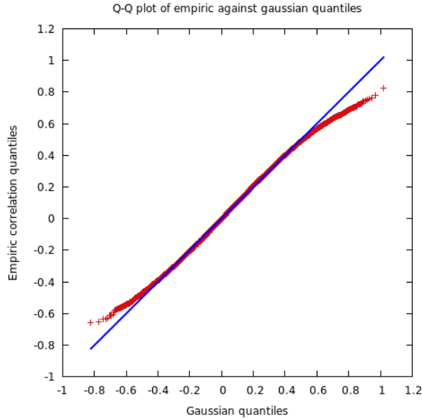
Figure 4: Q-Q plot of empiric against normal correlation quantiles for pairs of random CB -outranking relations of order 20
